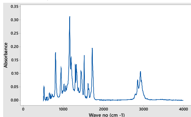
Fig. 7 FTIR graph for liquid monomer
