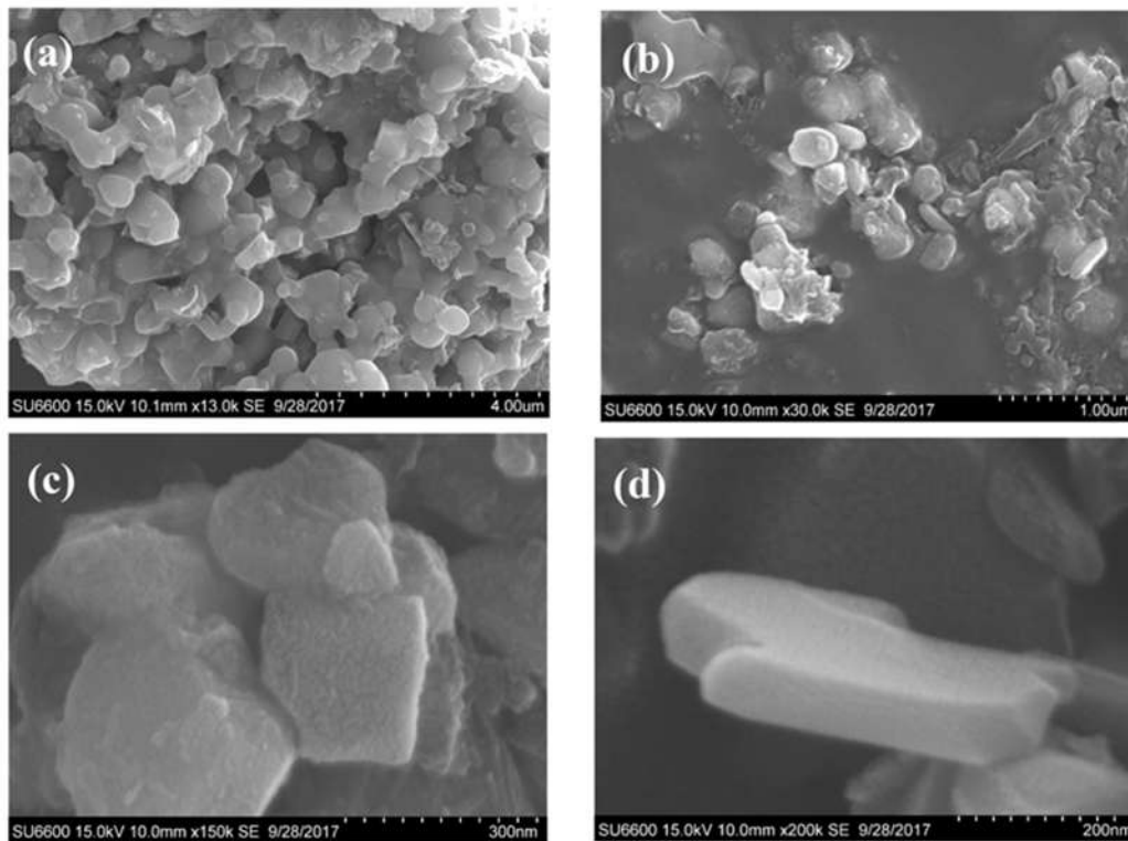
Figure 3. SEM images of hematite nanoparticles powder at (a) 4 \mu\text{m} , (b) 1 \mu\text{m} , (c) 300 nm, and (d) 200 nm magnifications, respectively.
