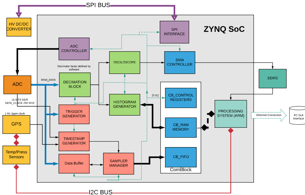
Figure 3: Functional diagram of the DAQ system implemented on the Zynq 7000 with peripherals. Timestamp and raw sample acquisition blocks are shown in red, signal analysis and diagnostic in light green, peripherals controllers in purple, FPGA-ARM communication in blue.
