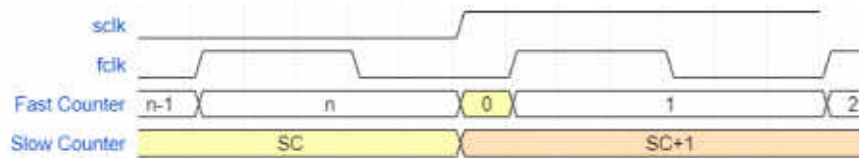
Figure 4: Time synchronization process
