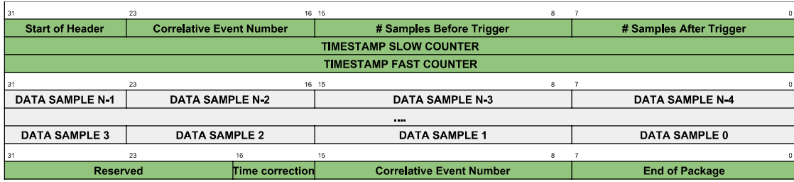
Figure 5: Package generated by Sampler Manager block stored on FIFO. .
