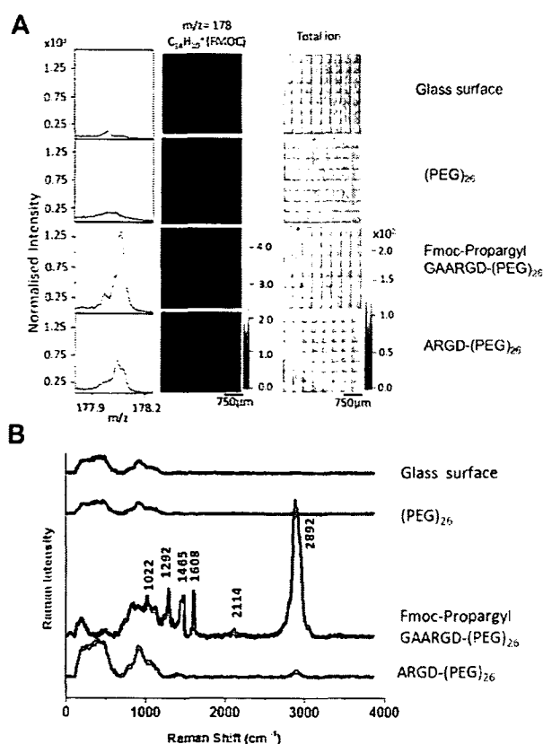
Fig. 2 (A) ToF-SIMS spectra and images of the Fmoc related ion fragment at m/z = 178 , ( C_{10}H_{14}^+ ) obtained from the samples before and after elastase treatment. The data was normalised to the total ion counts. (B) Raman spectra of enzyme responsive peptide surface (excitation wavelength- \lambda_{ex} = 532 nm, accumulation time 0.2 s).
