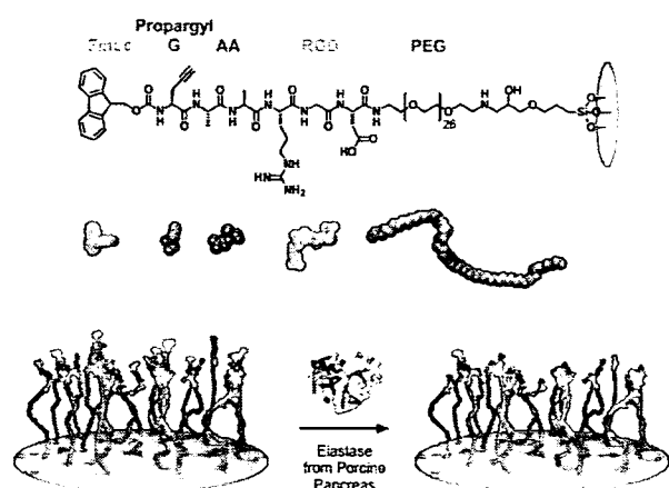
Fig. 1 The chemical structure of the peptides synthesized (top), cartoon representation of the elastase responsive peptide surface, Fmoc-propargyl-GAARGD-(PEG) 26 (bottom). After elastase exposure, the dialanine (AA) sequence is cleaved, removing Fmoc-propargyl GA and leaving ARGD-(PEG) 26 on the surface.
