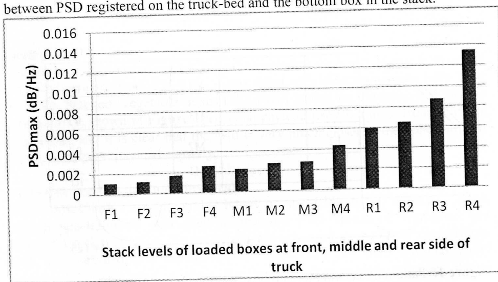
Figure 2. Summary of the results obtained on effective PSD levels of vertical vibration acceleration at different stack levels at front, middle, and rear of the truck bed. Average truck speed 20 \text{ kmh}^{-1} on fair road PSR 2 to 3 (or IRI 3.2 to 2 mm/m).
