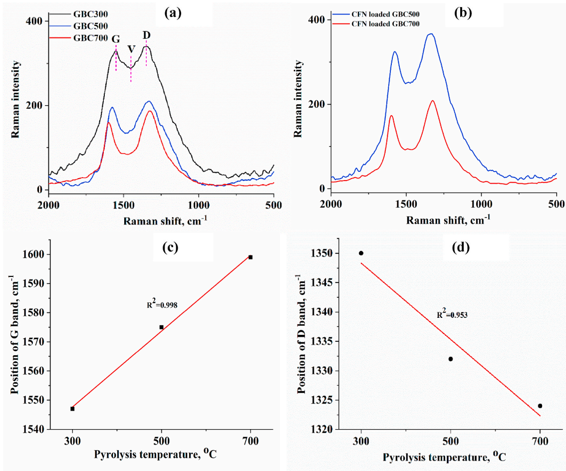
Fig. 4. The Raman spectra of pristine GBC (a) and CFN loaded GBC (b) and linear relationship between the position of G (c) and D (d) bands with pyrolysis temperature. Note: Raman spectrum of CFN loaded GBC300 is not reported above due to the fluorescence effect during the analysis.
