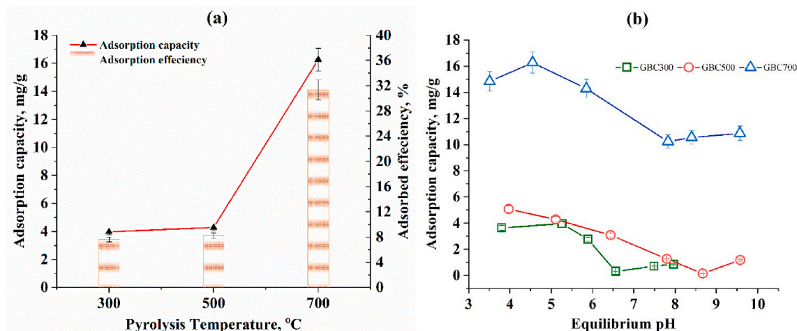
Fig. 5. The pattern of CFN adsorption capacity and CFN adsorption efficiency of GBC as the function of pyrolysis temperature (a) and the effect of pH on the CFN adsorption capacity at 25 ^{\circ}\text{C} (b). (The error bars represent the calculated \pm standard error of mean ( n = 3 )).
